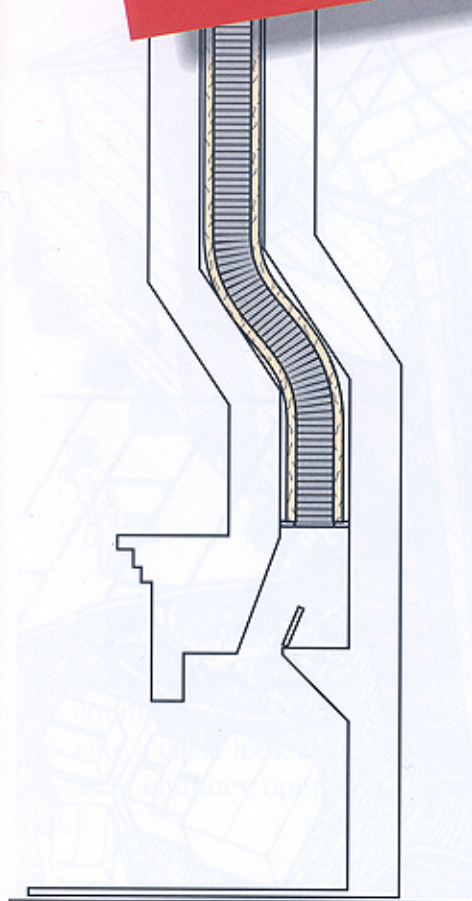
HomeSaver® is flexible to accommodate flue bends.
